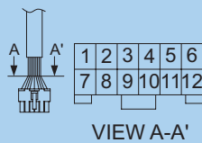
CONNECTOR : MOLEX 5557-12 (AC 전원용)
